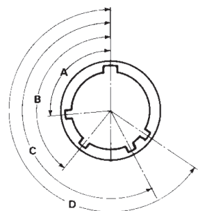
Viewed from front face of receptacle
