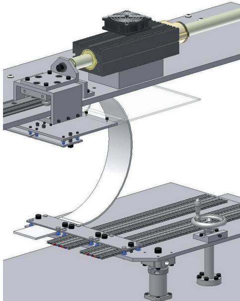
PART OF THE TEST EQUIPMENT DESIGNED BY AXON' CABLE
